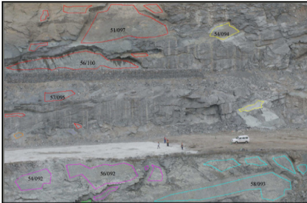
Figure 13 Dip and dip directions of a number of joints read off the SiroVision 3D image
