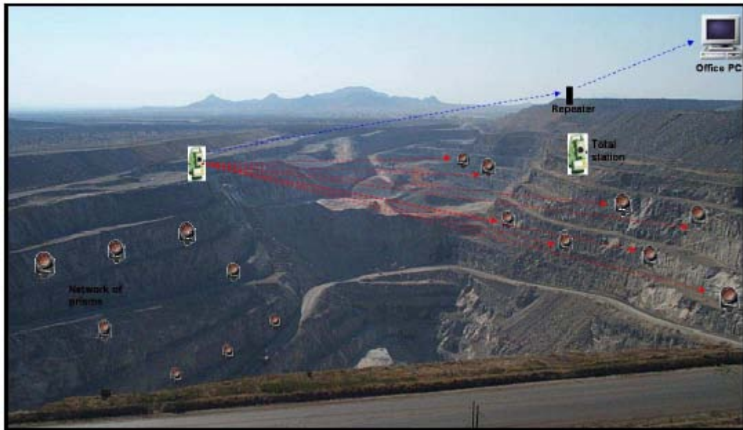
Figure 4 Prism network and monitoring setup in Sandsloot open pit
