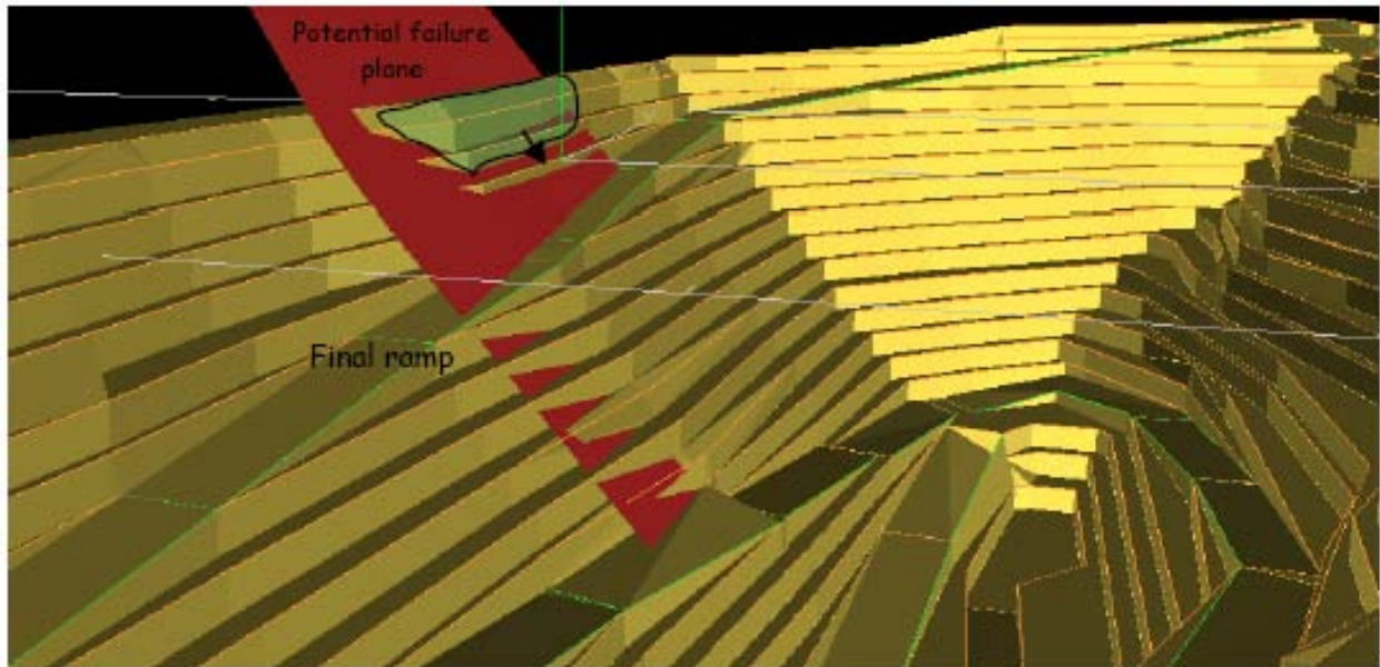
Figure 14 Failure plane measured in SiroJoint imported in Datamine and extrapolated on lower benches and ramps for stability analysis
