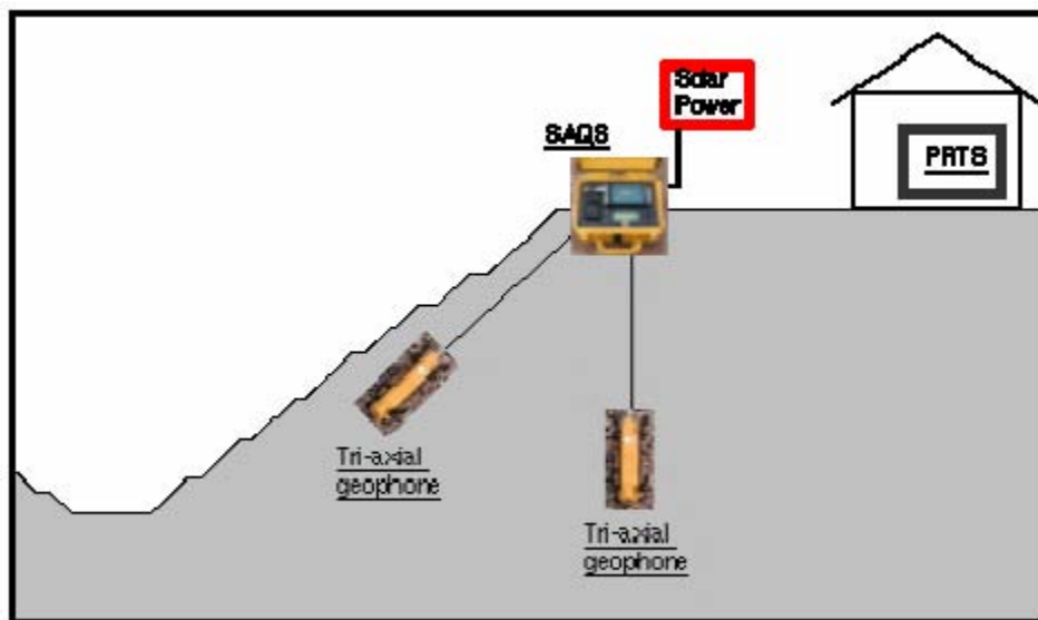
Figure 15 Sketch showing the setup of a seismic network in an open pit (ISSI website)
