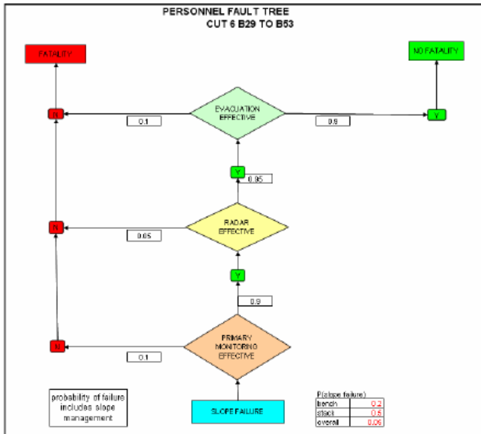
Figure 16 Fault tree design for Sandsloot open pit
