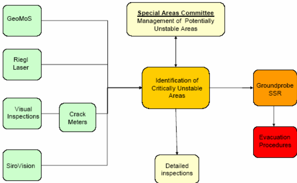
Figure 2 Slope monitoring strategy at PPRust
