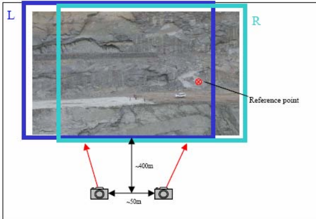
Figure 12 Method of obtaining photographs for SiroVision
