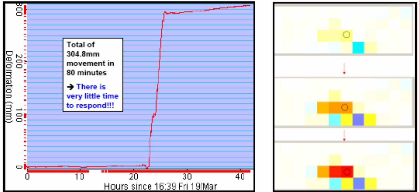
Figure 11 a) SSR deformation versus time plot of rapid brittle failure b) successive deformation images with change in colour showing the progressive movement
